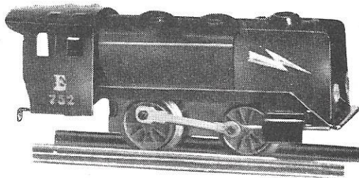
Lokomotiv, 165 mm.
